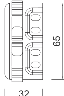
2'li Multi Klips Düşey Vertical Multi Clips with 2 head
