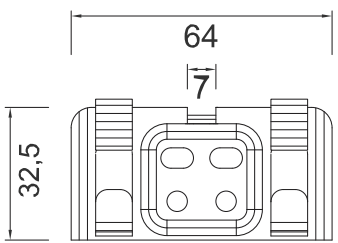
2'li Multi Klips Yatay Horizontal Multi Clips with 2 head
